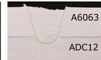
Excellent Joint Cross Section
